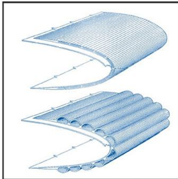
Goodrich pneumatic boots
