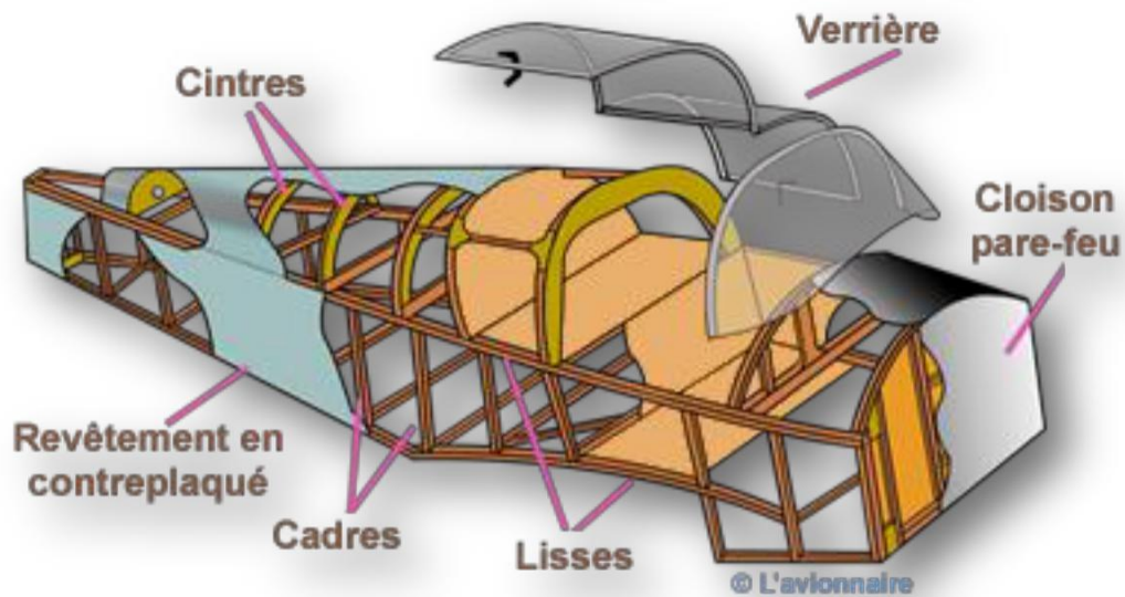
Structure Bois
